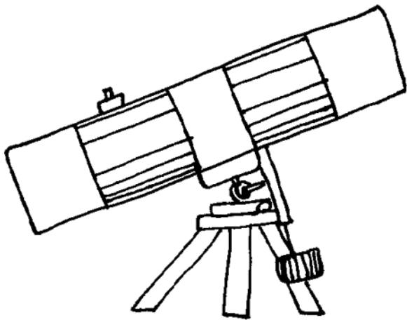
telescope
